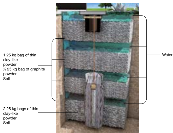
APPLICATION AT-070H
